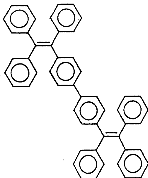
4,4'-bis[(1,2,2-trisphenyl)ethenyl]-biphenyl
